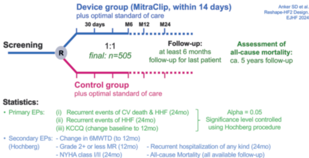
Figure 3. Trial design of RESHAPE-HF2 – testing transcatheter edge-to-edge repair (MitraClip) in the 3 rd population, using the Hochberg procedure for primary and secondary endpoints.
