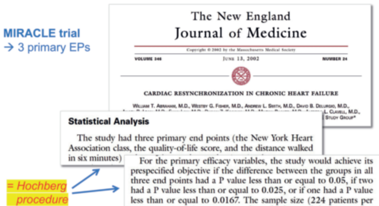
Figure 2. Historical example of using the Hochberg procedure for 3 primary endpoints in a clinical trial in chronic heart failure. Examples are screen shots of Abraham et al. , NEJM 2002 8
